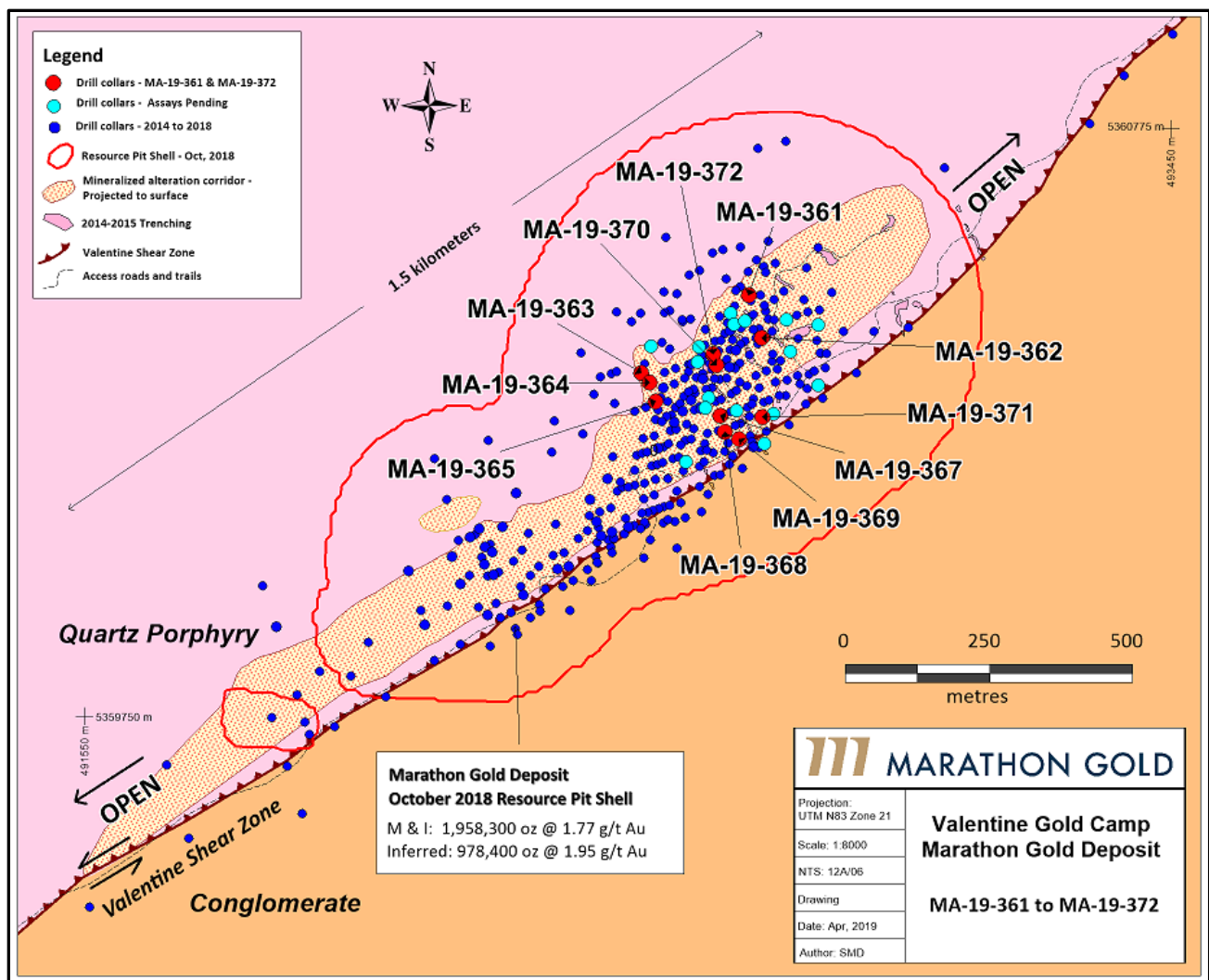
Figure 1: Location of drill hole collars MA-19-361 to MA-19-372, Marathon Deposit.
