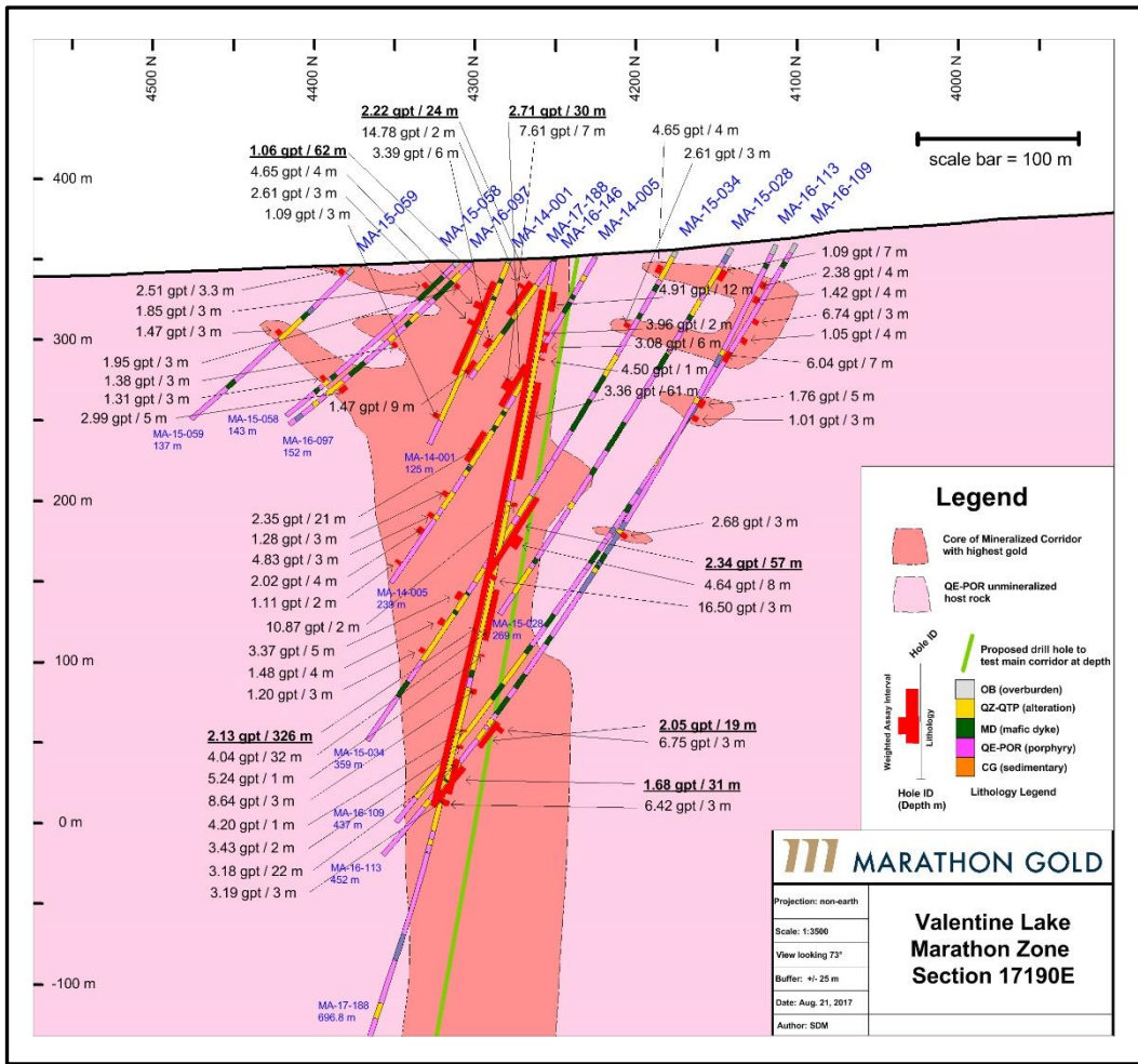
Figure 2: Cross Section 17190E Marathon Deposit
