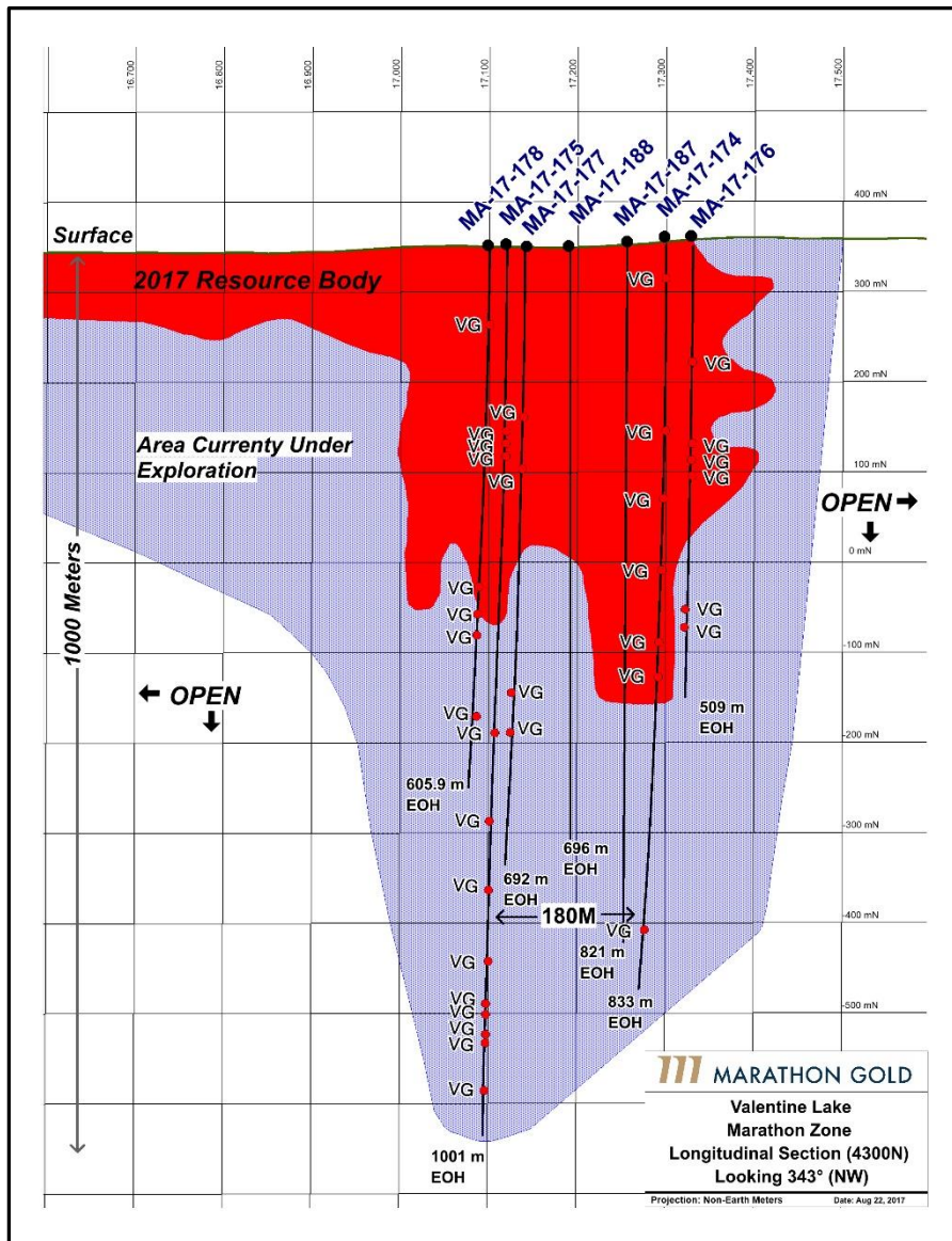
Figure 3: Long Section 4300N Marathon Zone
