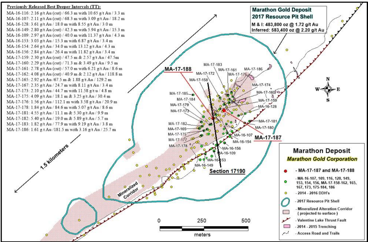
Figure 1: Location map showing the new drill holes MA-17-187 and MA-17-188, Marathon Deposit
